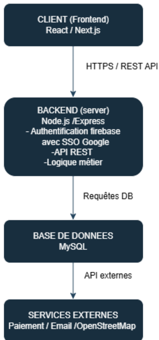
Figure 3.1 Architecture de la plateforme
